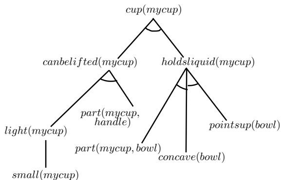
Fig. 13.11 Explanation-based learning to identify the object cup
