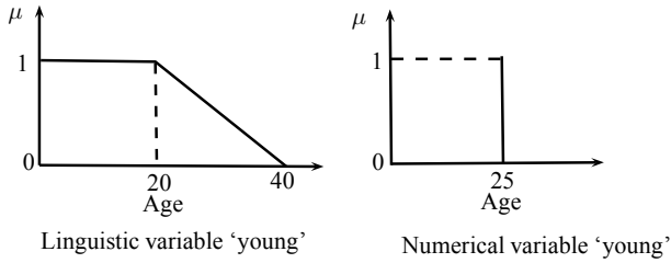
Fig. 12.14 Linguistic and numerical variable “young”
