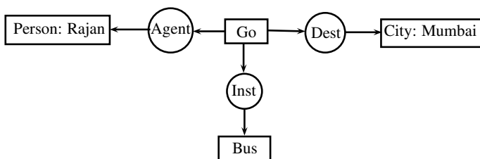
Fig. 7.5 Conceptual Graph-II
