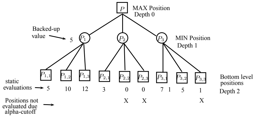
Fig. 11.15 Alpha-beta search
