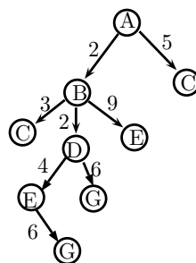
(b) Search-Tree.
