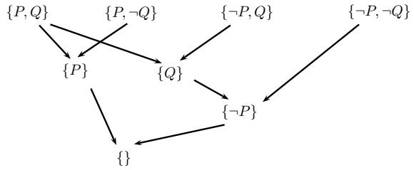
Fig. 3.2 DAG for theorem proving
