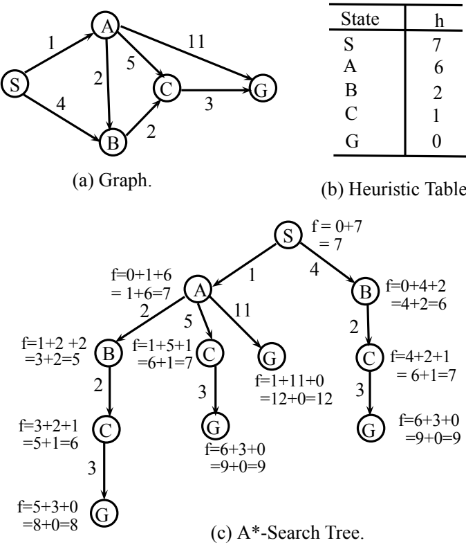
Fig. 9.5 Graph and A*-Search tree
