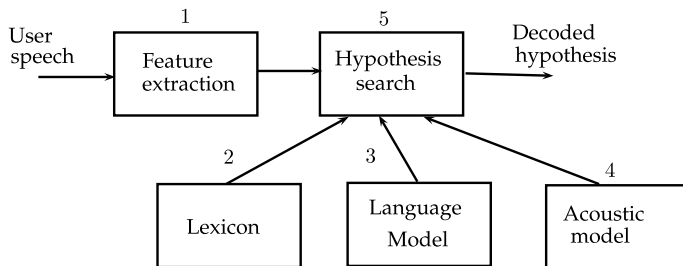
Fig. 20.3 Speech recognition system block diagram
