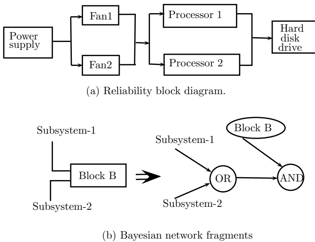
Fig. 12.11 Syntheizing a Bayesian network
