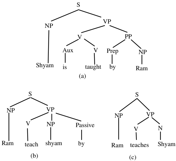
Fig. 19.5 Transformational Grammar
