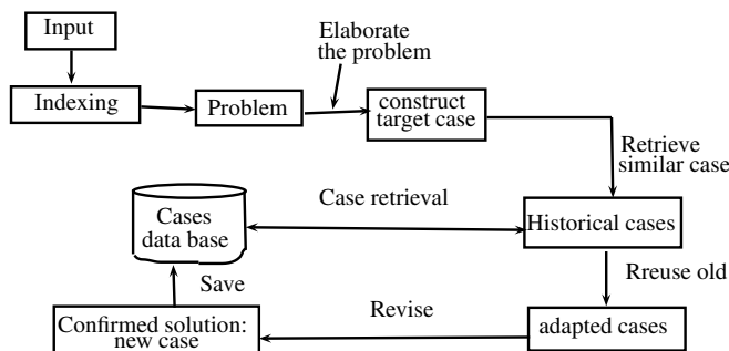
Fig. 4.3 Case-based Reasoning
