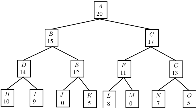
Fig. 8.8 State—space tree
