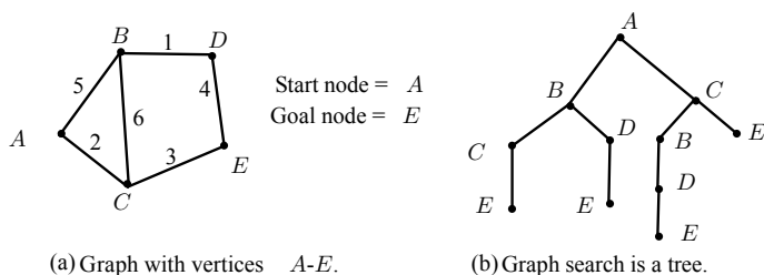
Fig. 8.2 Undirected graph
