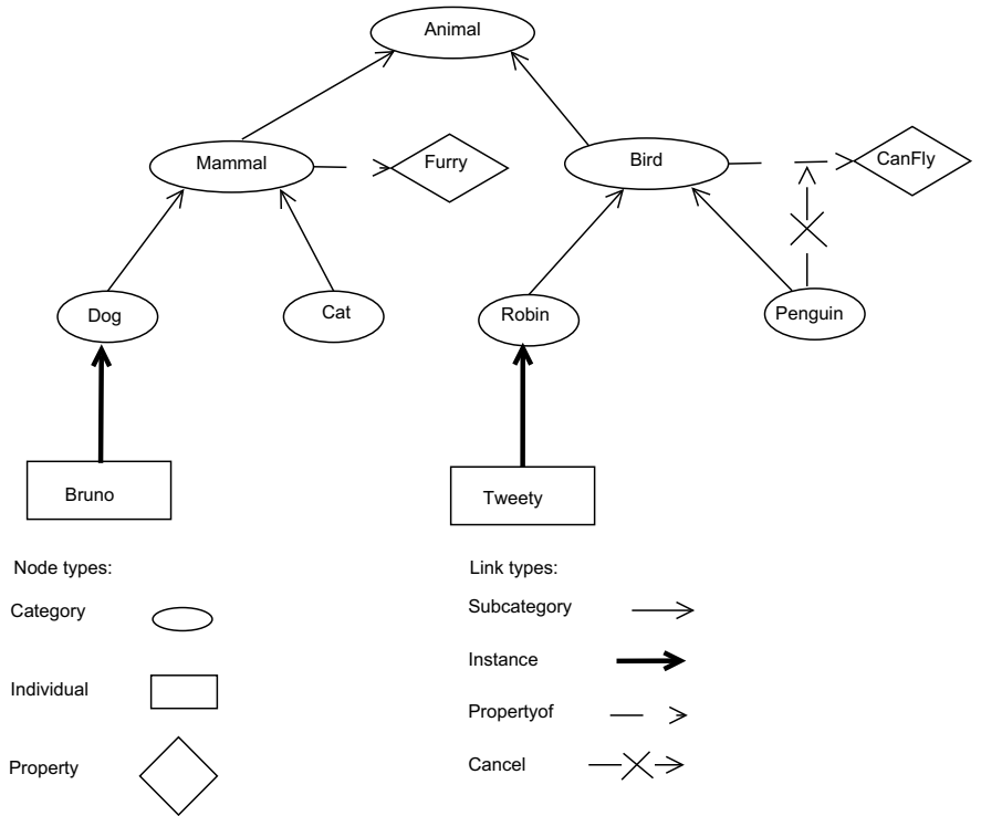
Fig. 6.1 Taxonomy of animal world
