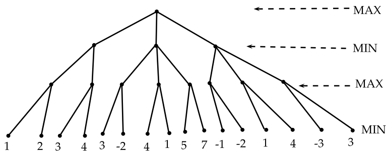
Fig. 11.18 Game-tree
