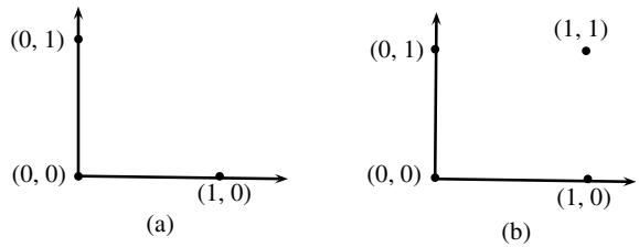
Fig. 14.12 Training data for SVMs
