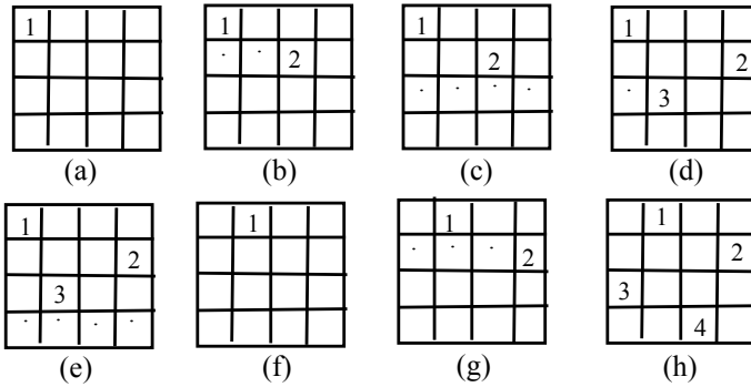
Fig. 10.9 Backtrack based solution for four queens Problem
