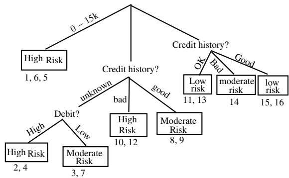
Fig. 13.5 Learning through decision tree
