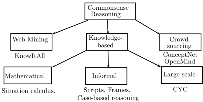
Fig. 6.2 Taxonomy of approaches to commonsense reasoning
